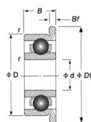
Open type
