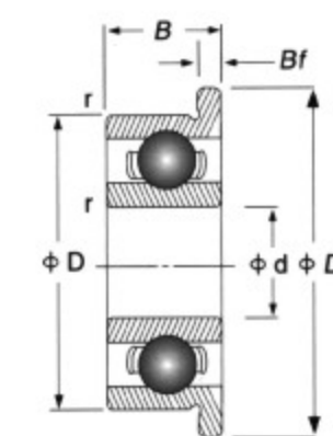
Open type
