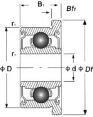
Shielded type(ZZ)
