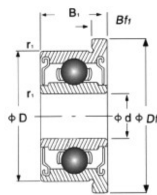
Shielded type(ZZ)
