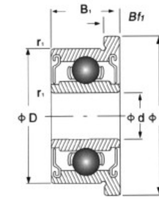
Shielded type(ZZ)
