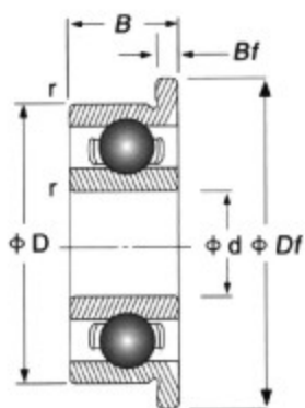
Open type
